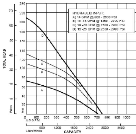
S4VHL Typical Performance
