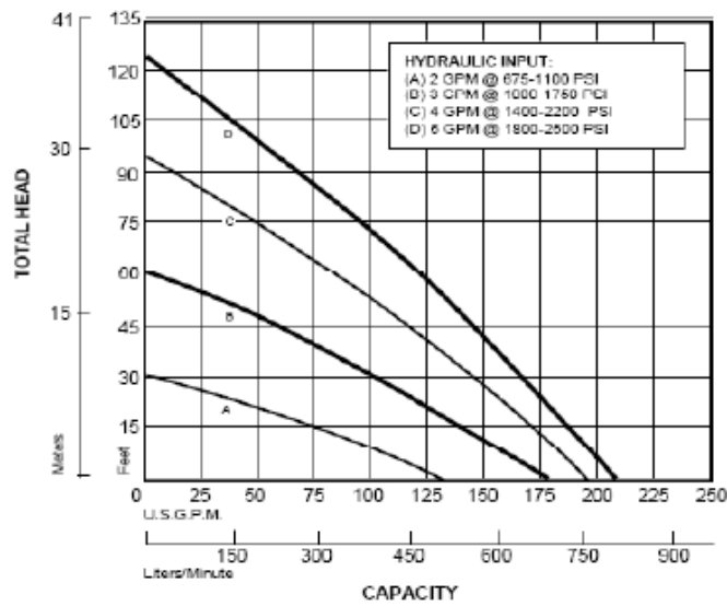
S2TC-2 Typical Performance
