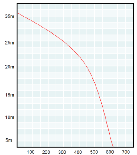
200mm (8") Liquidator
