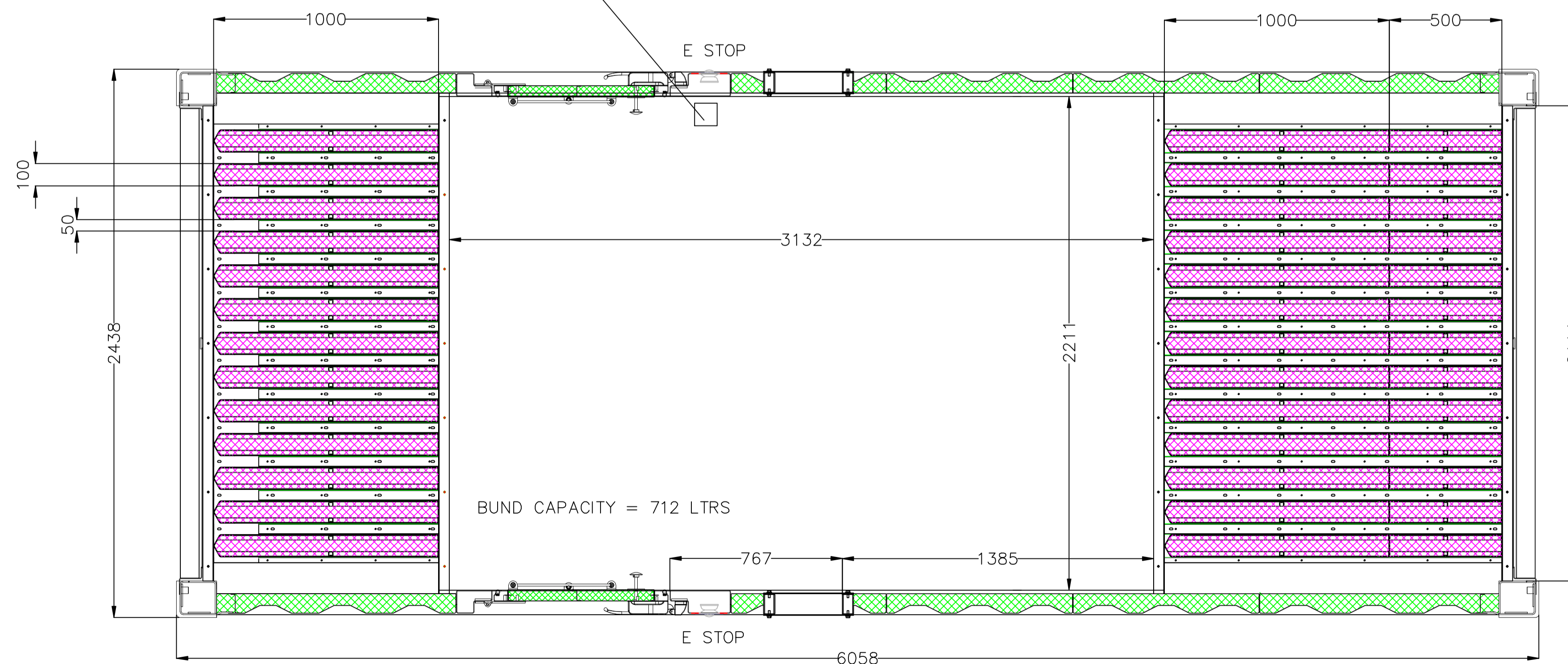
PLAN VIEW (ROOF DETAIL REMOVED)
