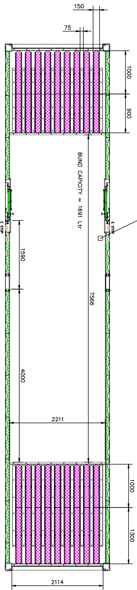
PLAN VIEW (ROOF DETAIL REMOVED)
